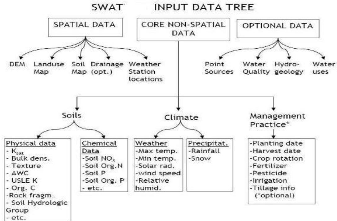
Fig. 1: Overview on required input information for SWAT (from [4])
